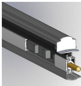
* Slide Bolt Astragal
