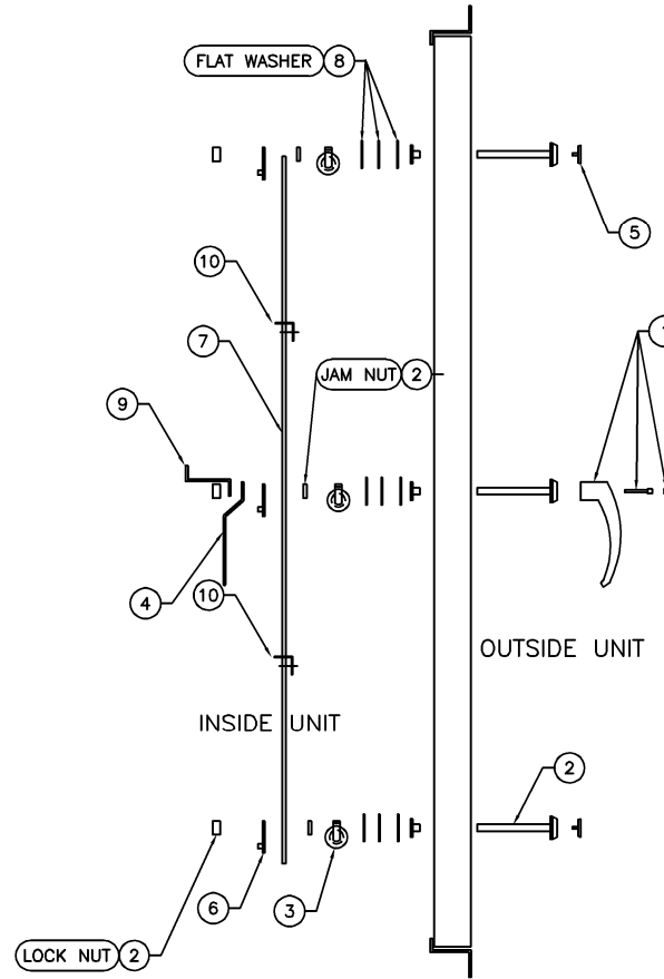
STANDARD DOOR MULTI-POINT OUT SWING 3 LATCHES
