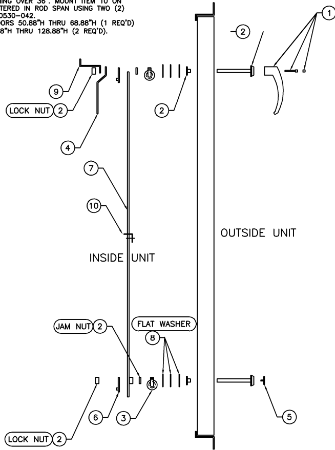
STANDARD DOOR MULTI-POINT OUT SWING 2 LATCHES
